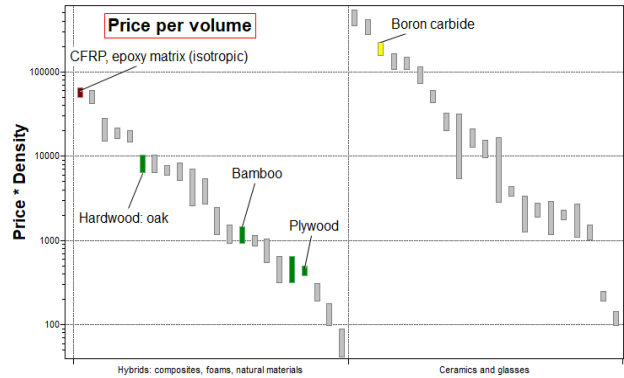
Chart: Boron carbide (and CFRP) usually have very good performance but are also very expensive. Wood costs less.
